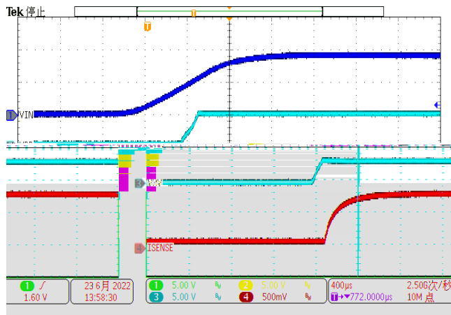
Figure 12. Power Up
